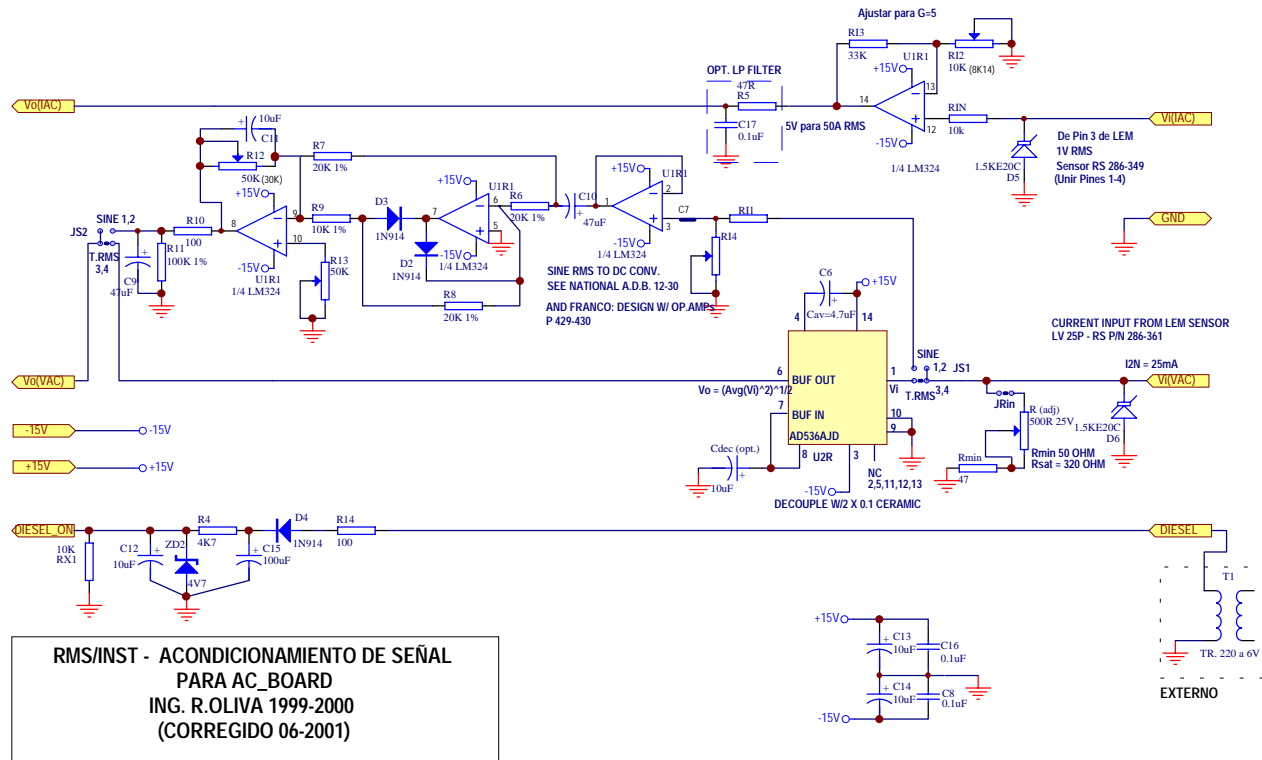
Figure 2 - Typical AC Board Signal Conditioning
